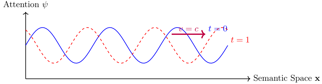
Wave propagation: Ideas spread at velocity c
